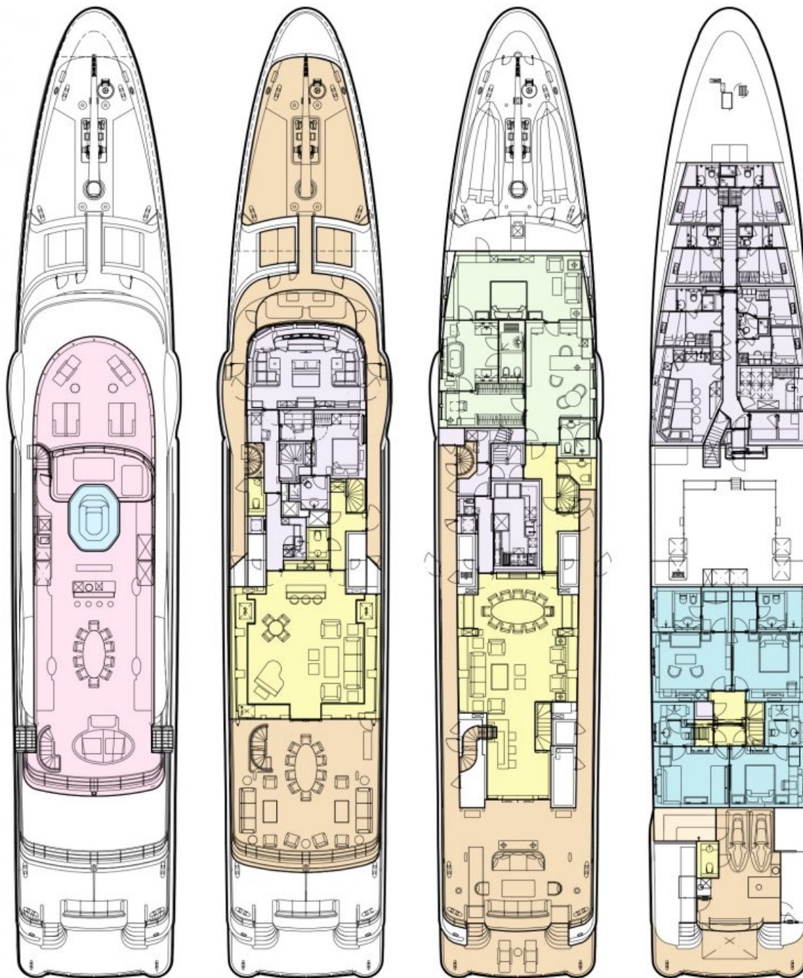
STEP ONE, 180' (55.00m) Amels Motoryacht, 2012
